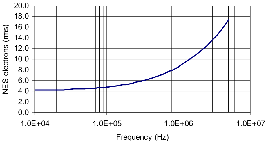
Estimated Read Noise (BI)
