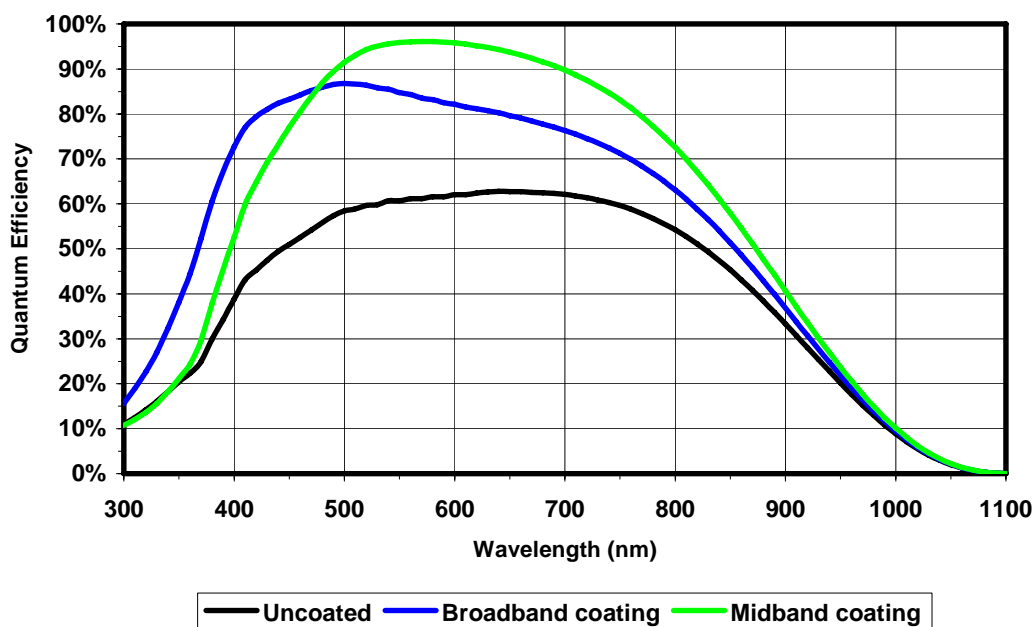
Typical QE at -25C
