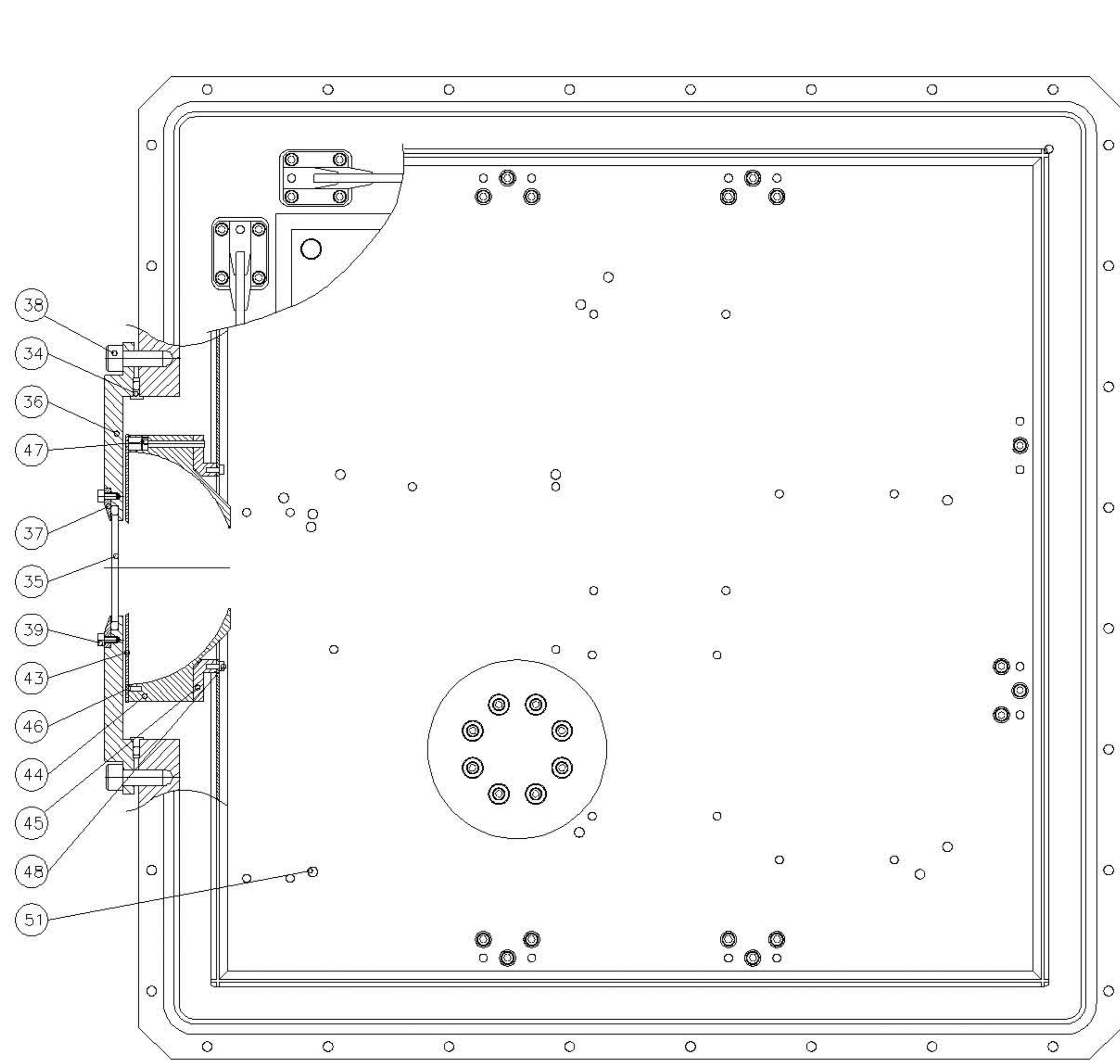
VIEW MAIN FLANGE
