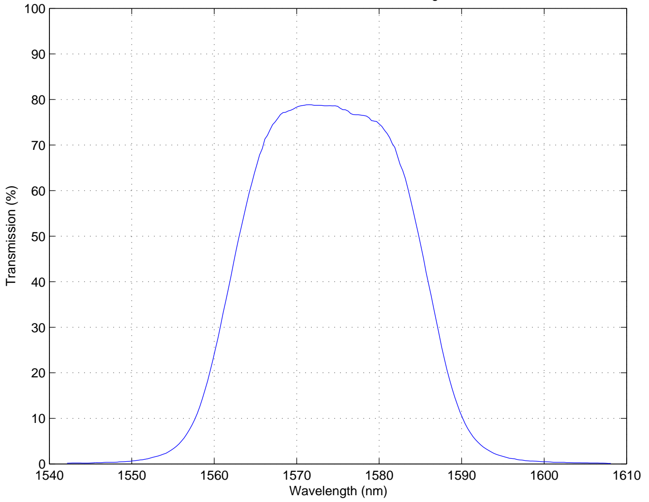
Filter #211, H-continuum, vacuum wavelength, T=74K
