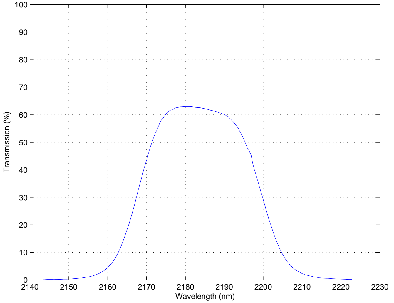
Filter #219, He 1c, vacuum wavelength, T=74K
