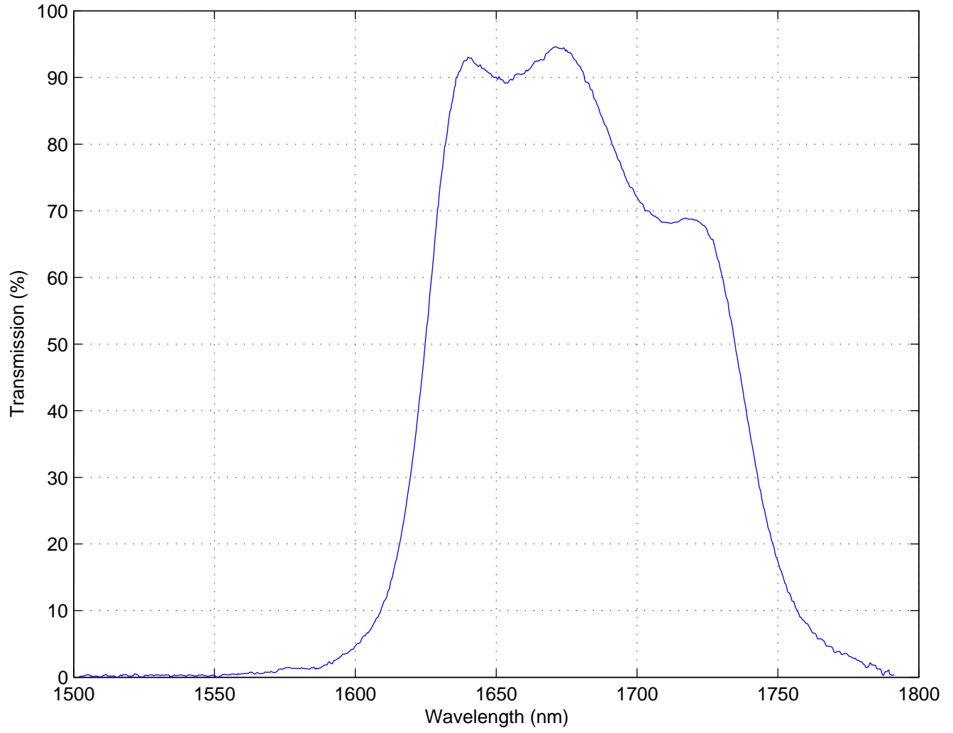
Filter #224, CH4 I, vacuum wavelength, T=74K
